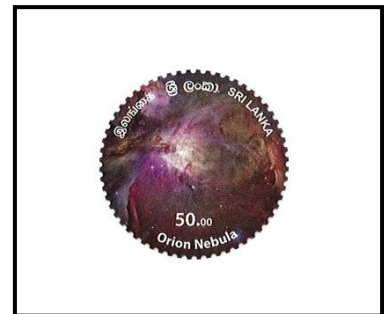
Orion Nebula
