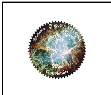
Crab Nebula
