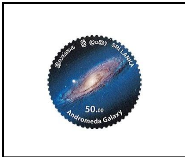
Andromeda
