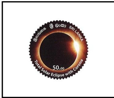
Solar Eclipse
