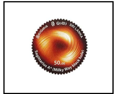
Black Hole
